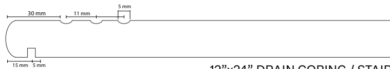
12"x24" DRAIN COPING / STAIR
